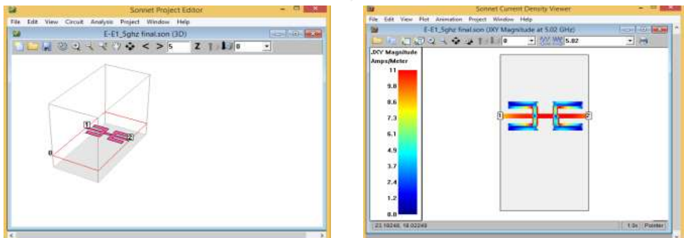
Fig.2.Three Dimension of Patch Antenna Array & its Current Density of Patch Antenna Array
