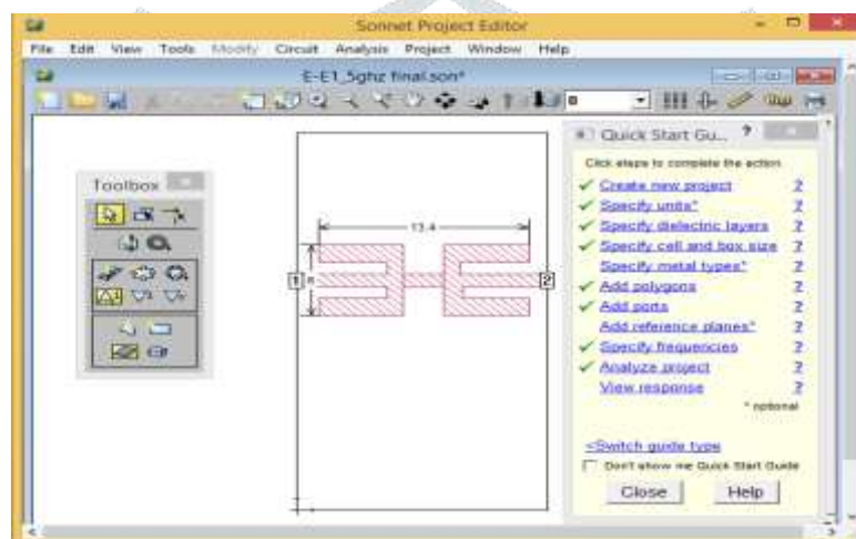
Figure.1. Geometry of E-Shaped Patch Antenna Array
