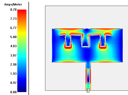
Figure 5.2 Current Distribution at 4.95GHz
