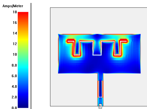
Figure 5.1 Current Distribution at 2.525GHz
