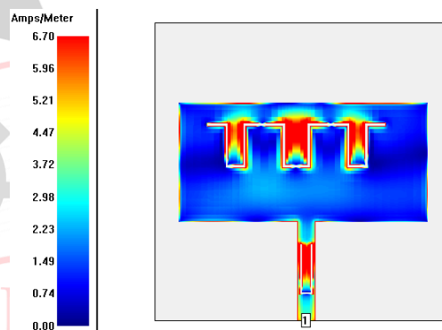
Figure 5.4 Current Distribution at 7.0GHz
