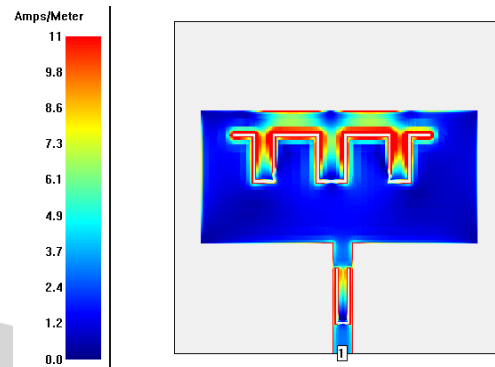
Figure 5.3 Current Distribution at 6.525GHz
