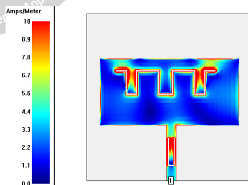
Figure 5.5 Current Distribution at 9.55GHz
