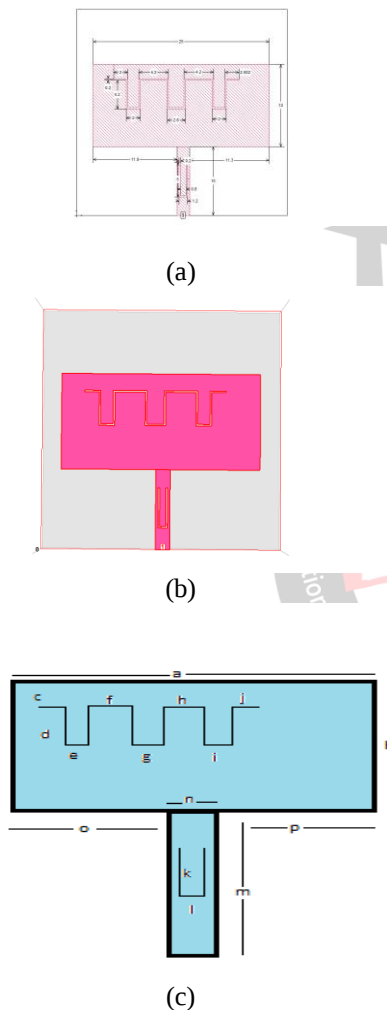
Figure 1: Geometry of the Multiband Antenna
